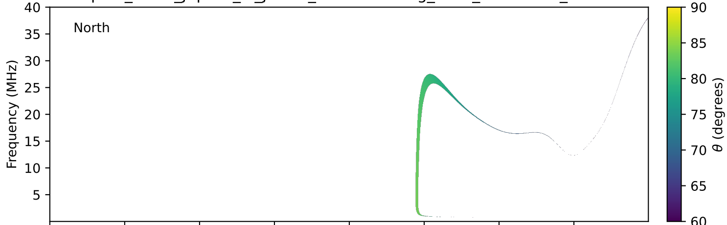
expres_earth_jupiter_io_jrm33_lossc-wid1deg_3kev_19910418_v11.cdf
