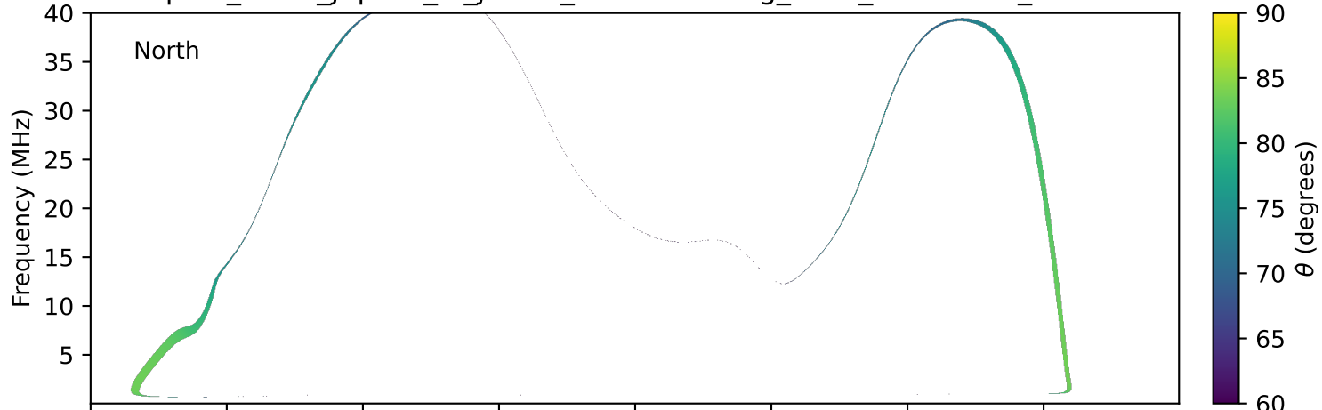
expres_earth_jupiter_io_jrm33_lossc-wid1deg_3kev_19910415_v11.cdf
