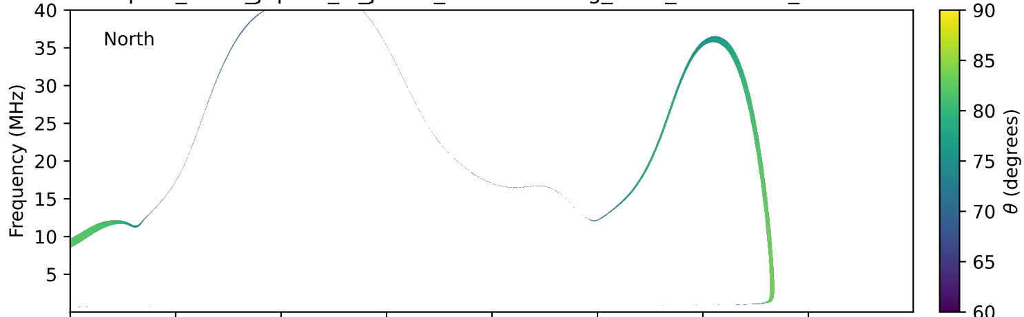
expres_earth_jupiter_io_jrm33_lossc-wid1deg_3kev_19910408_v11.cdf
