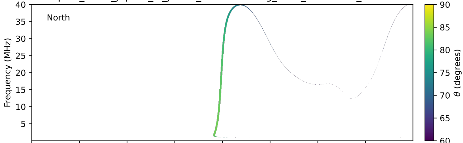
expres_earth_jupiter_io_jrm33_lossc-wid1deg_3kev_19910404_v11.cdf
