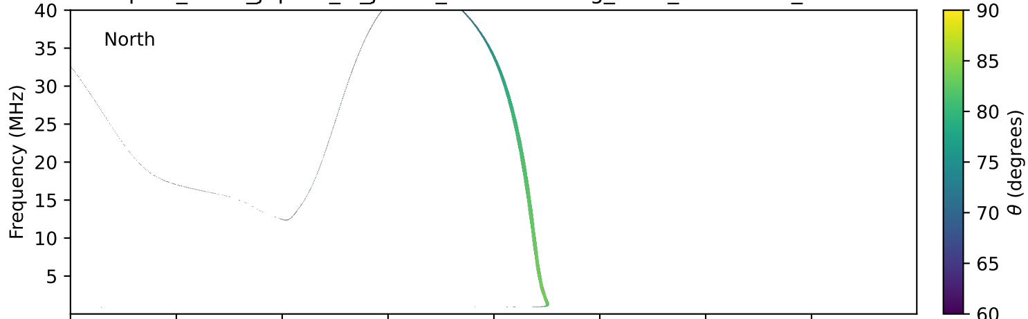
expres_earth_jupiter_io_jrm09_lossc-wid1deg_3kev_19910410_v11.cdf
