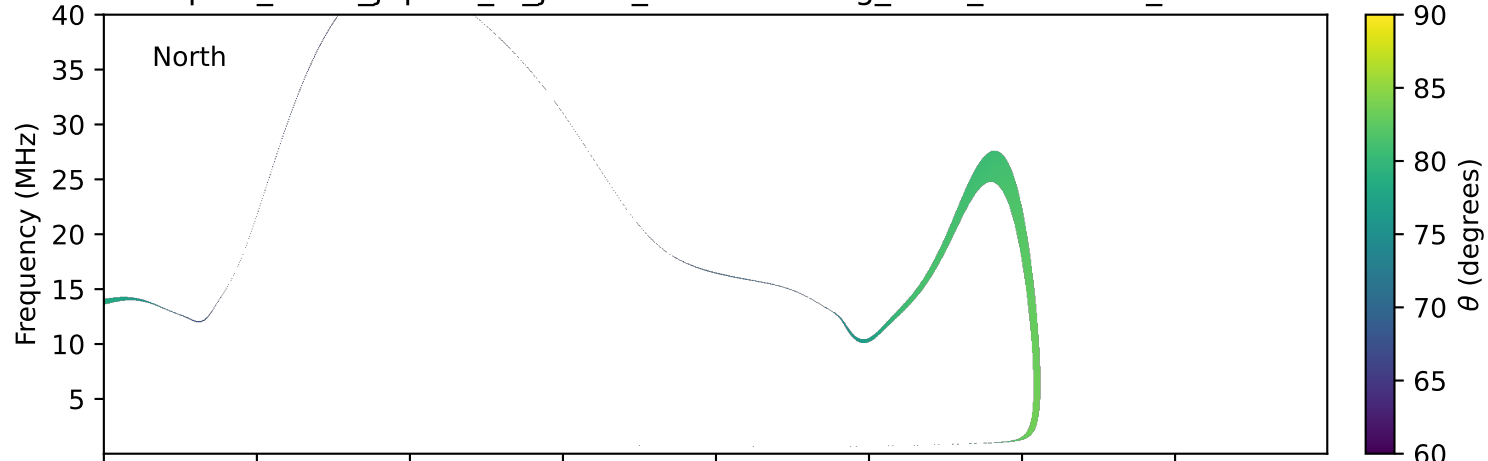
expres_earth_jupiter_io_jrm09_lossc-wid1deg_3kev_19910401_v11.cdf
