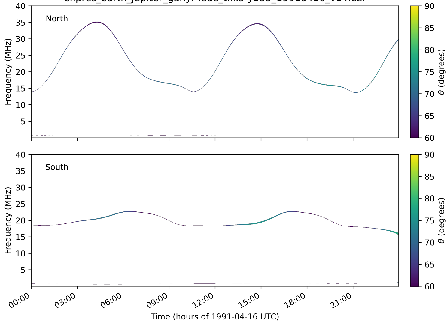
expres_earth_jupiter_ganymede_txka-y235_19910416_v14.cdf
