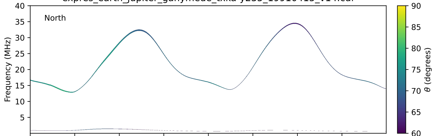
expres_earth_jupiter_ganymede_txka-y235_19910415_v14.cdf
