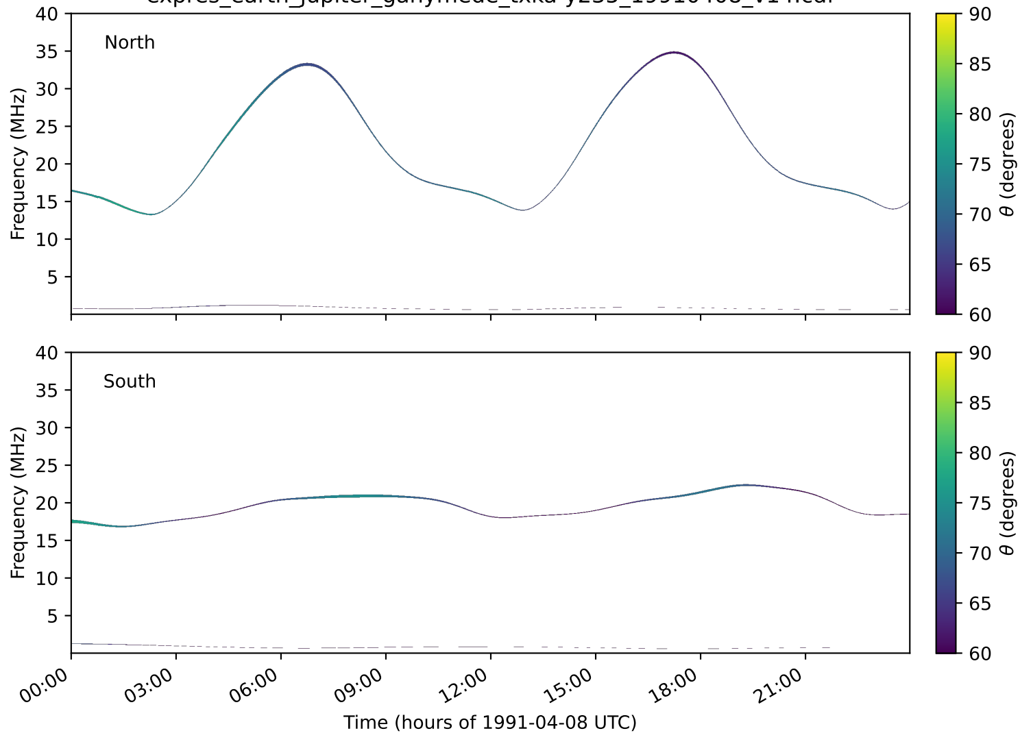
expres_earth_jupiter_ganymede_txka-y235_19910408_v14.cdf
