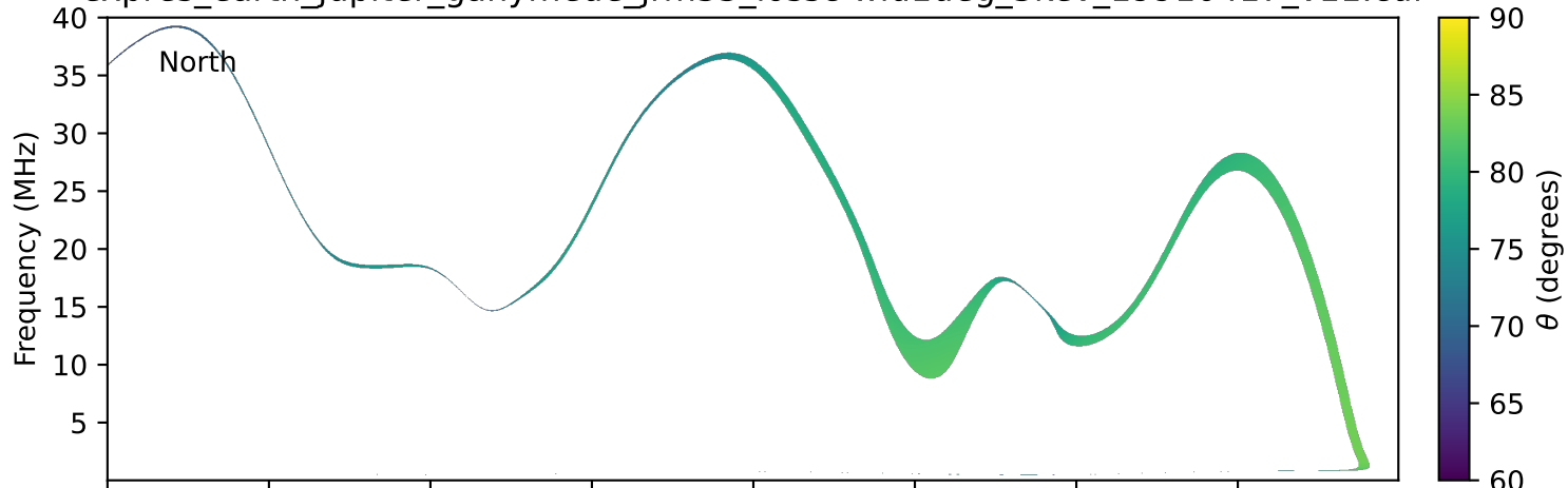
expres_earth_jupiter_ganymede_jrm33_lossc-wid1deg_3kev_19910417_v11.cdf
