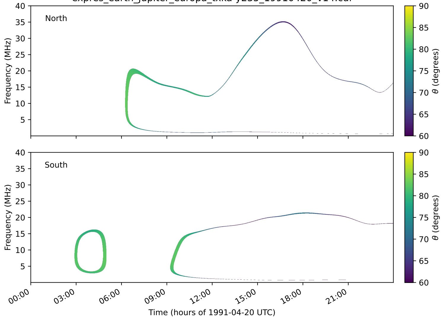
expres_earth_jupiter_europa_txka-y235_19910420_v14.cdf
