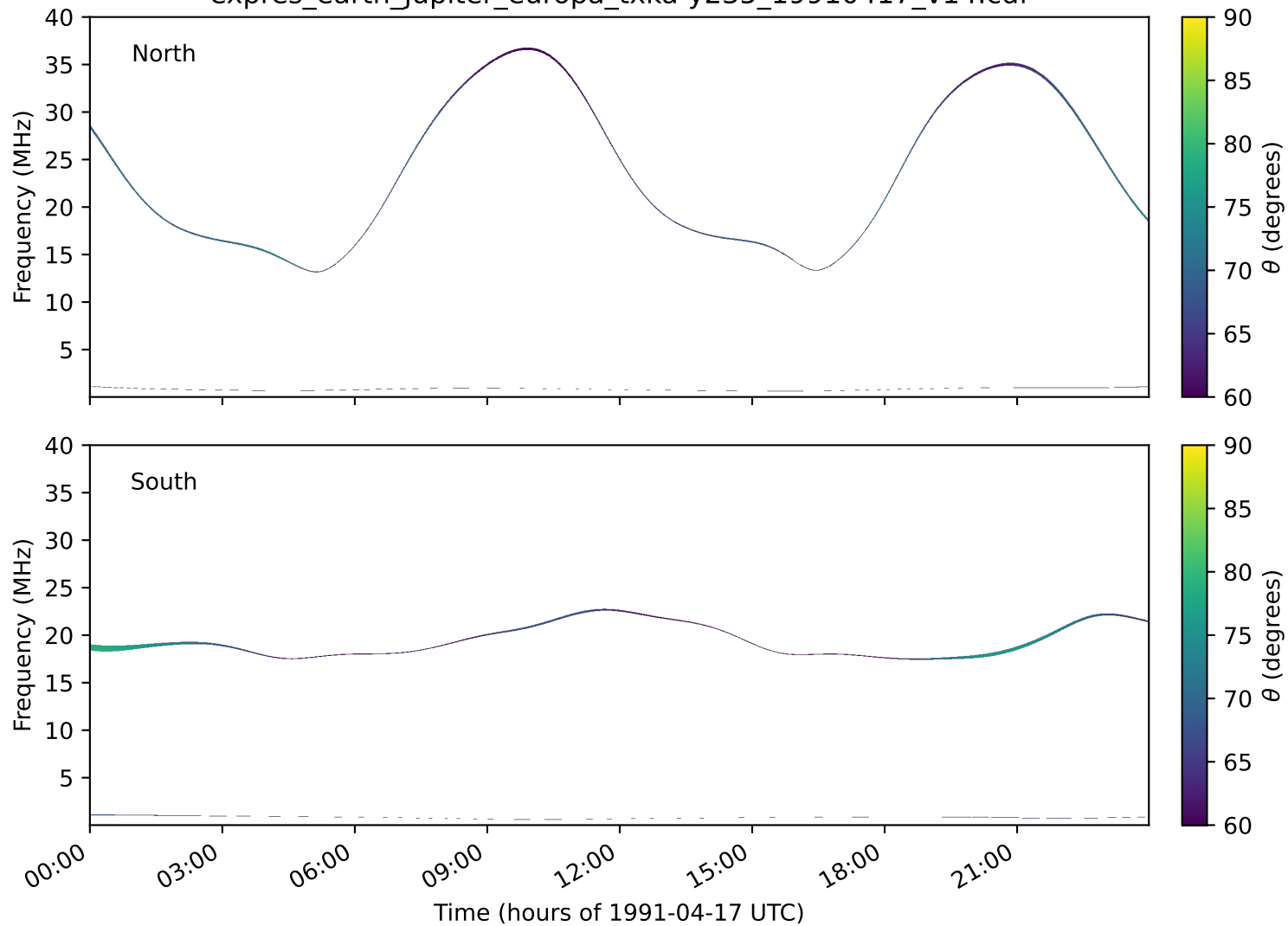
expres_earth_jupiter_europa_txka-y235_19910417_v14.cdf
