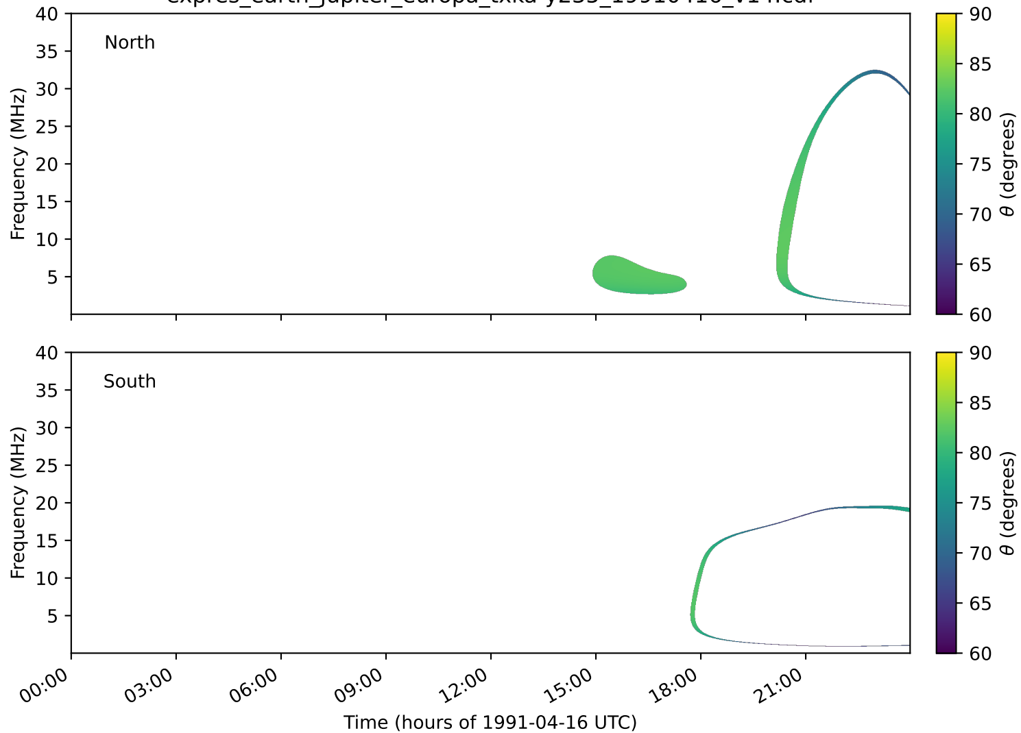
expres_earth_jupiter_europa_txka-y235_19910416_v14.cdf
