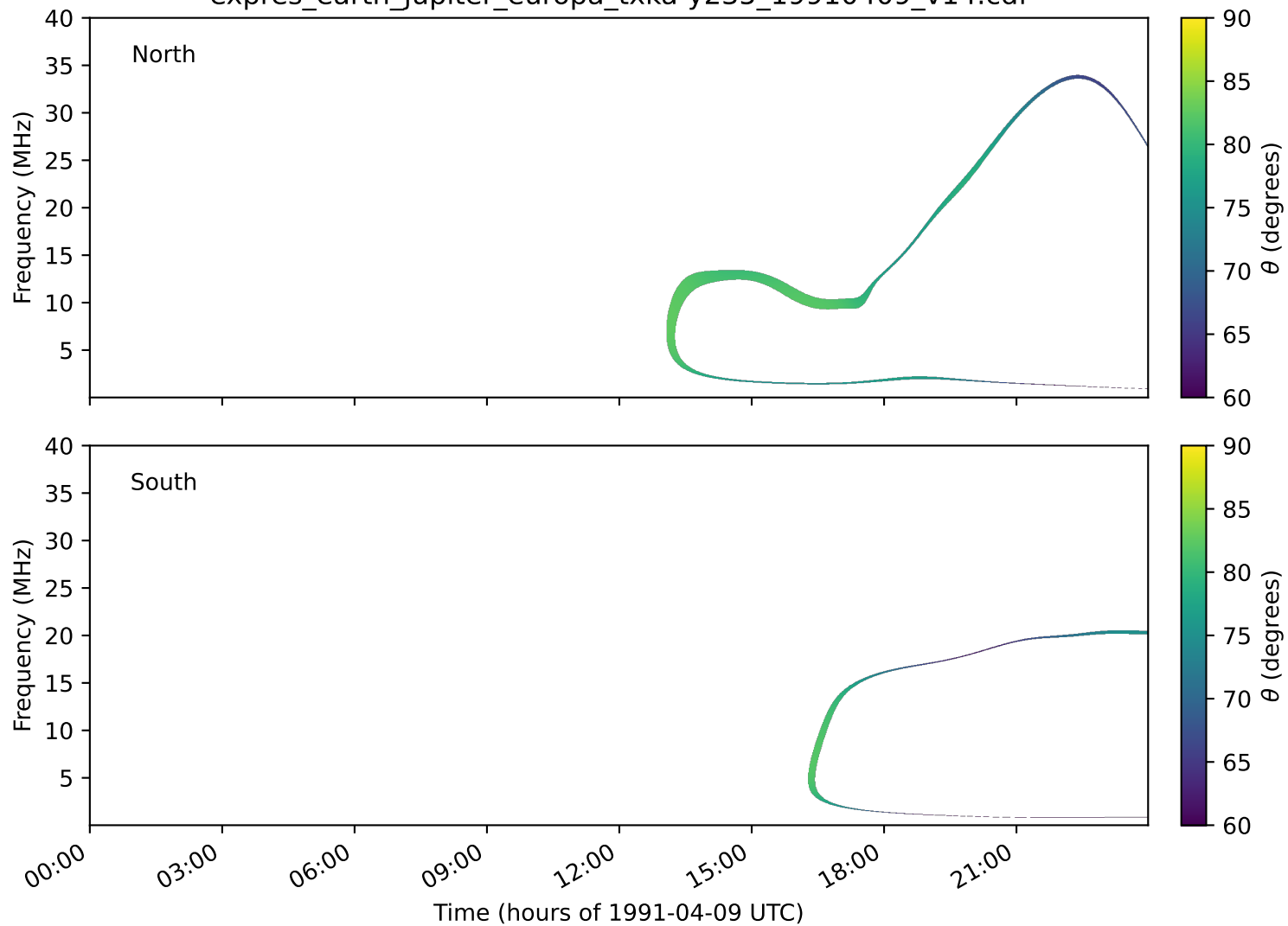
expres_earth_jupiter_europa_txka-y235_19910409_v14.cdf
