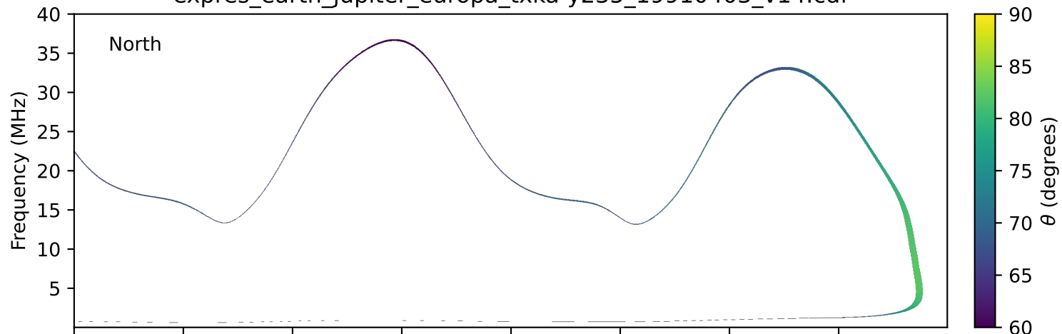
expres_earth_jupiter_europa_txka-y235_19910403_v14.cdf
