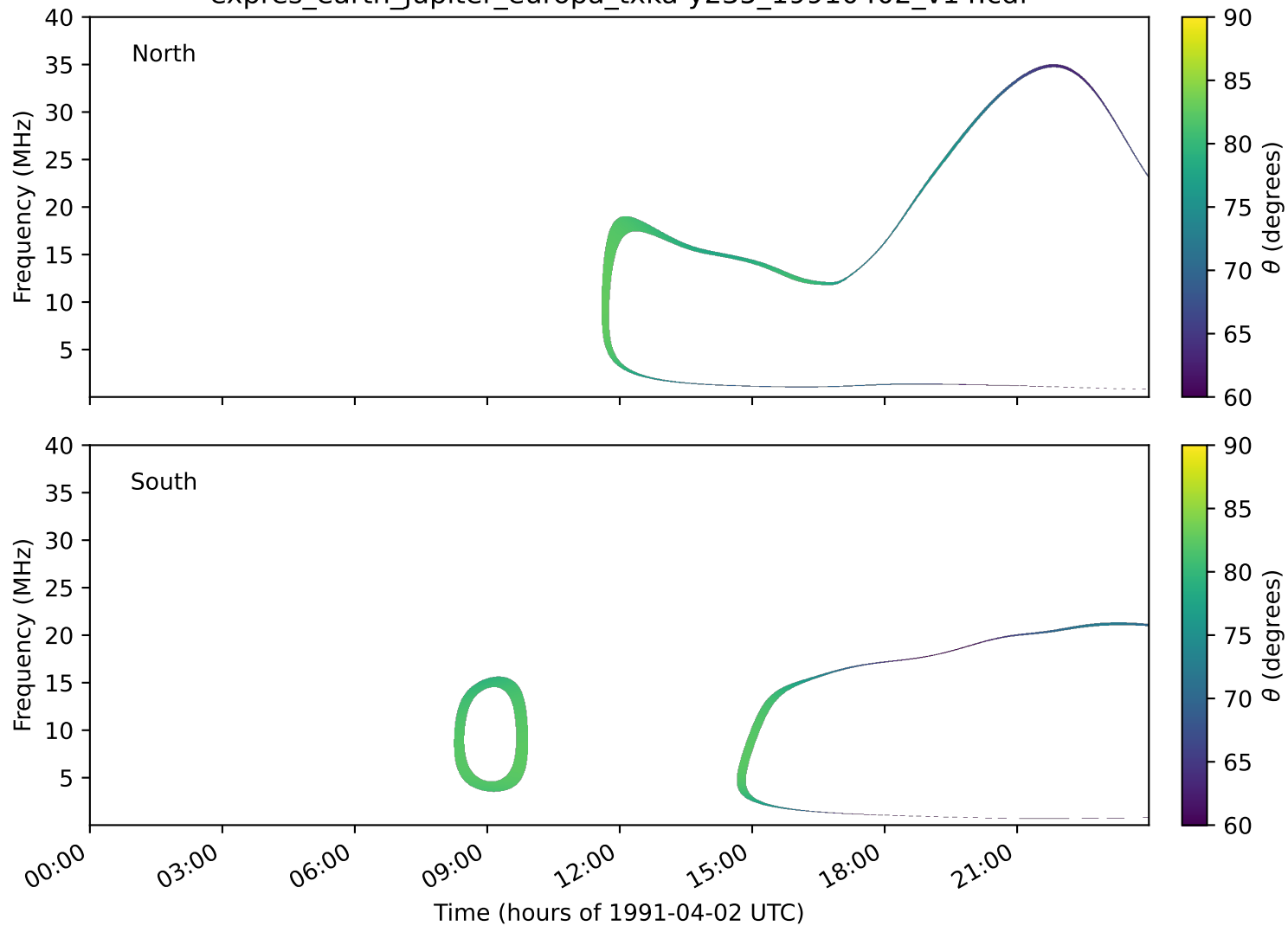
expres_earth_jupiter_europa_txka-y235_19910402_v14.cdf
