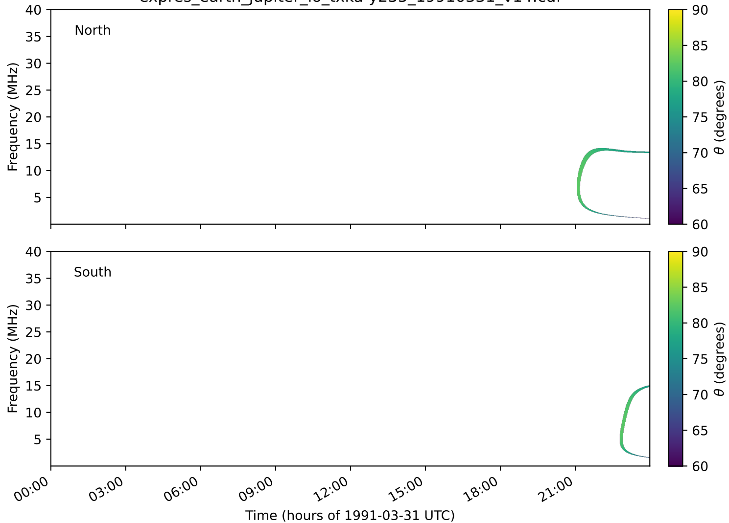
expres_earth_jupiter_io_txka-y235_19910331_v14.cdf
