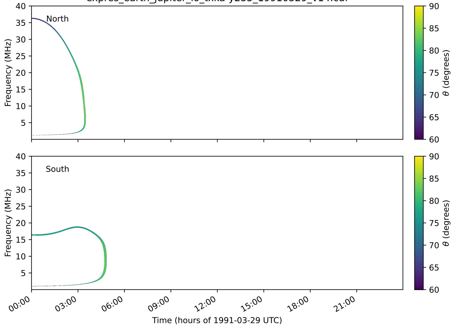
expres_earth_jupiter_io_txka-y235_19910329_v14.cdf
