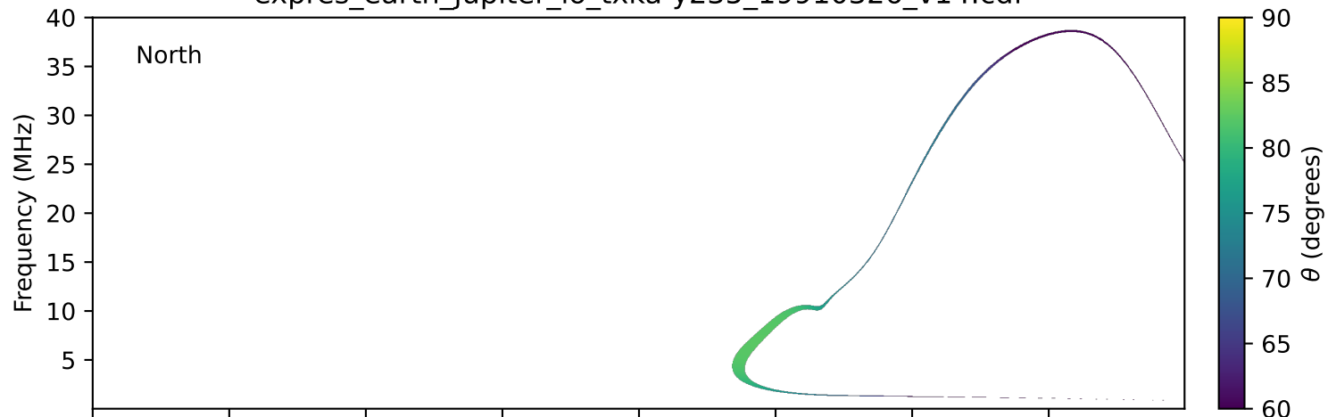
expres_earth_jupiter_io_txka-y235_19910326_v14.cdf
