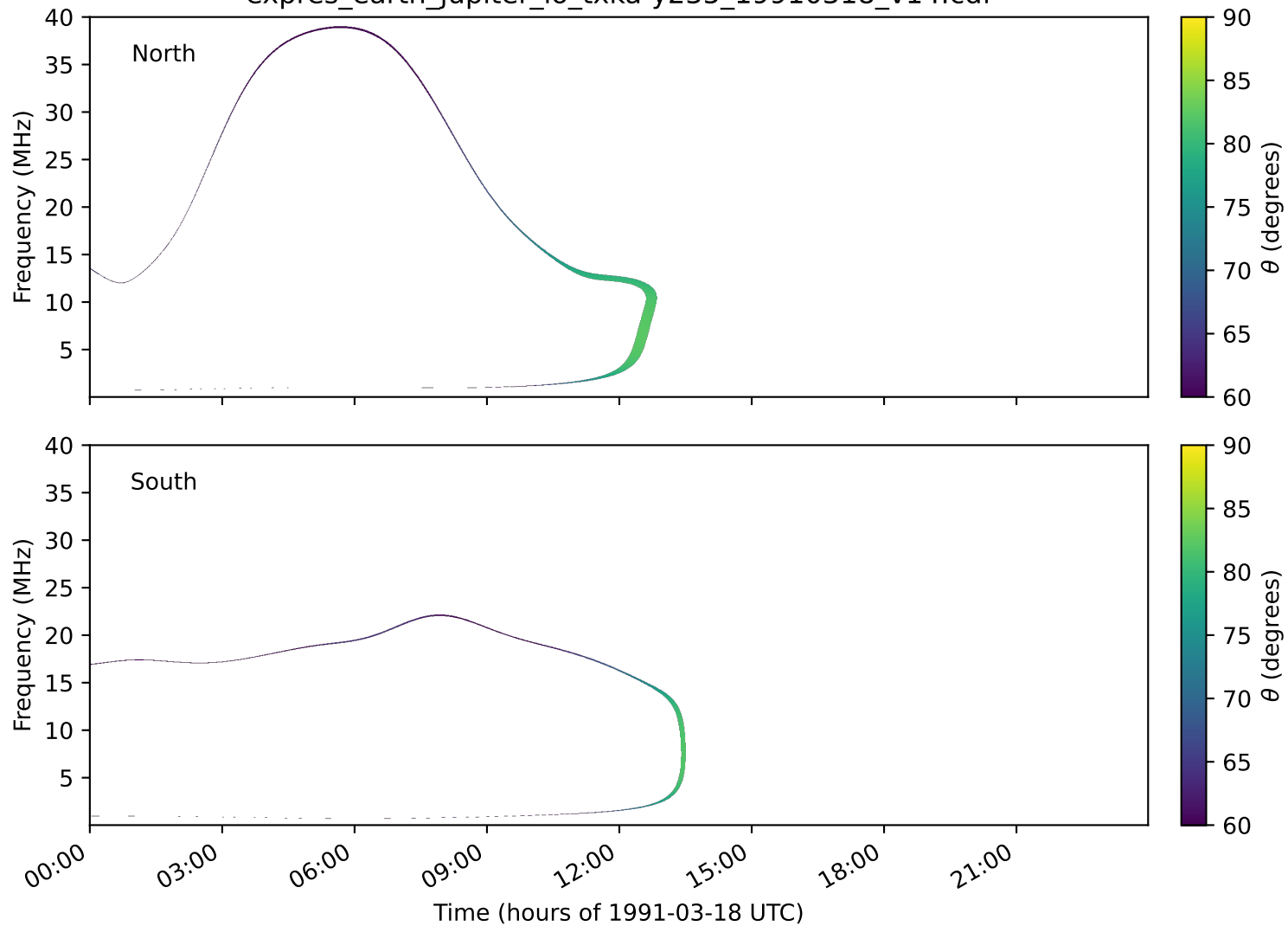
expres_earth_jupiter_io_txka-y235_19910318_v14.cdf
