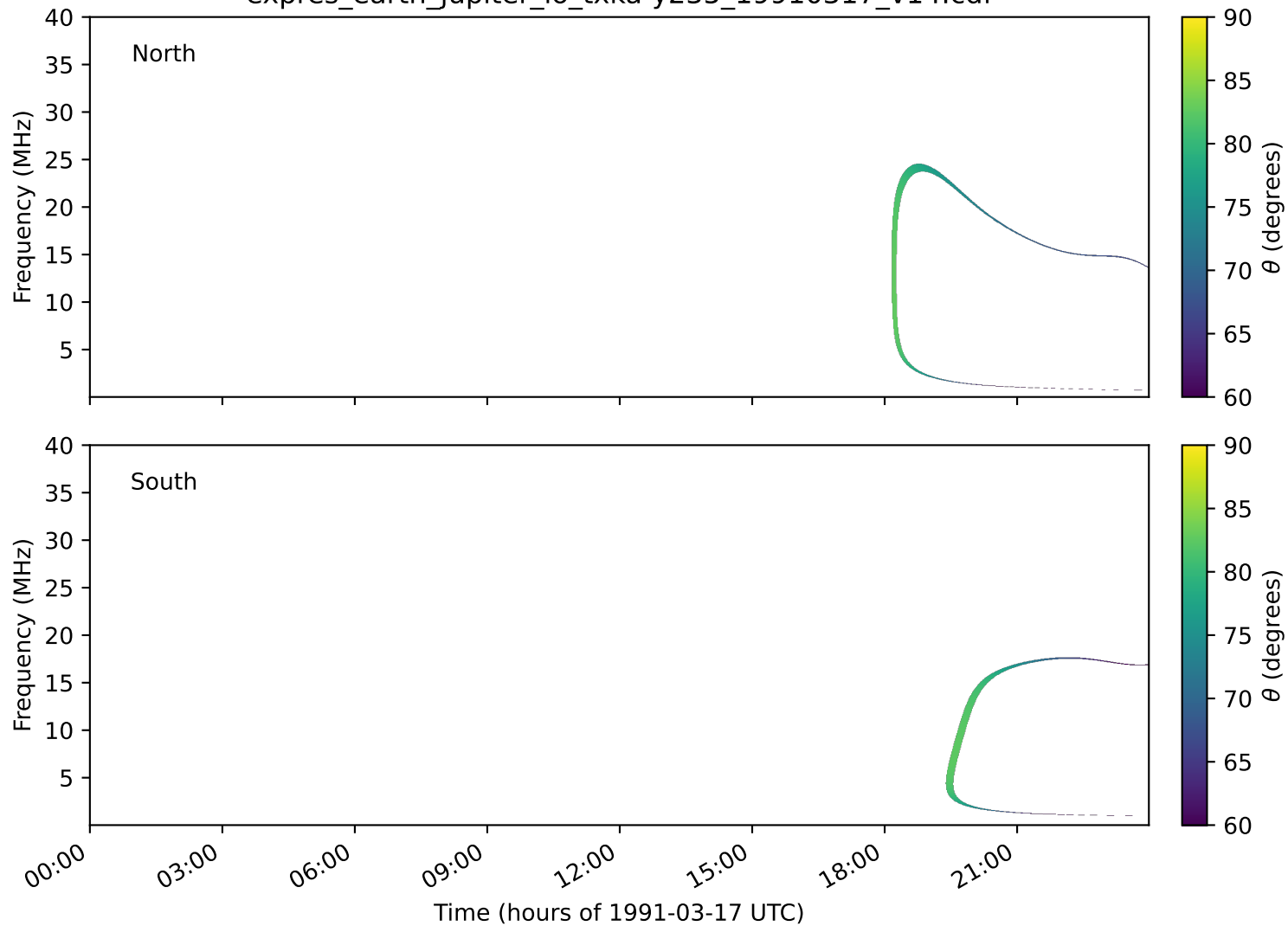
expres_earth_jupiter_io_txka-y235_19910317_v14.cdf
