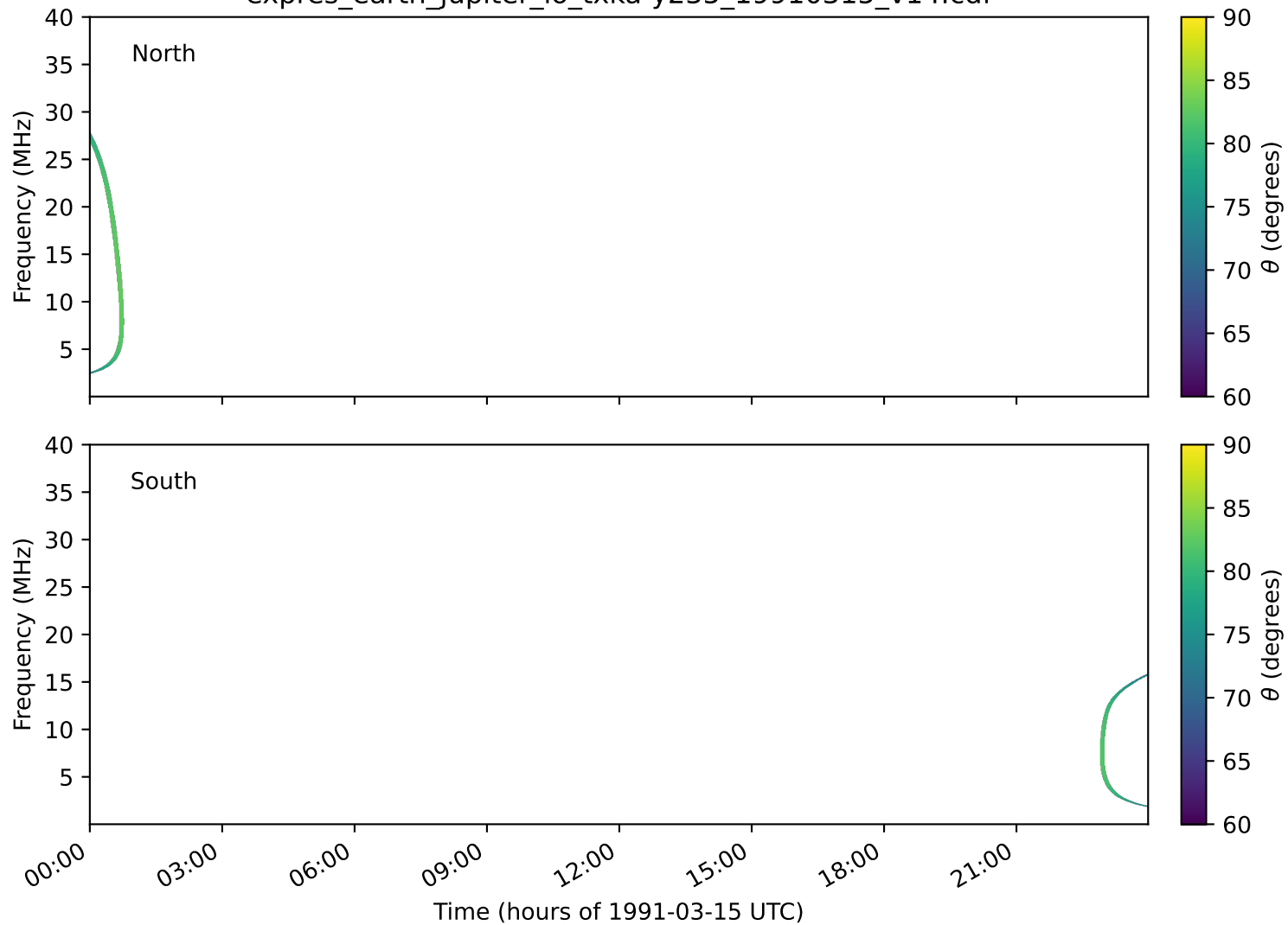
expres_earth_jupiter_io_txka-y235_19910315_v14.cdf
