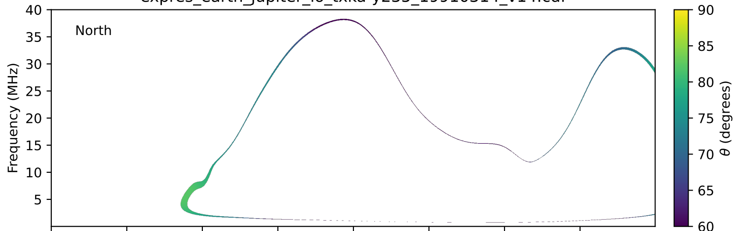
expres_earth_jupiter_io_txka-y235_19910314_v14.cdf
