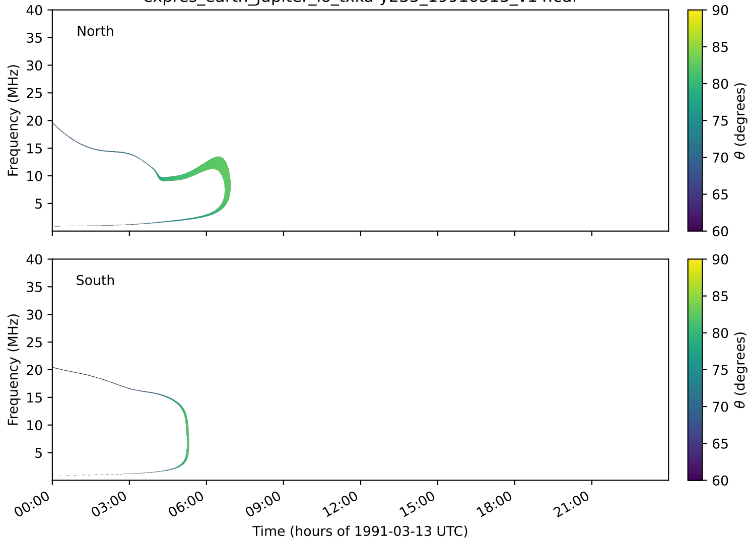
expres_earth_jupiter_io_txka-y235_19910313_v14.cdf
