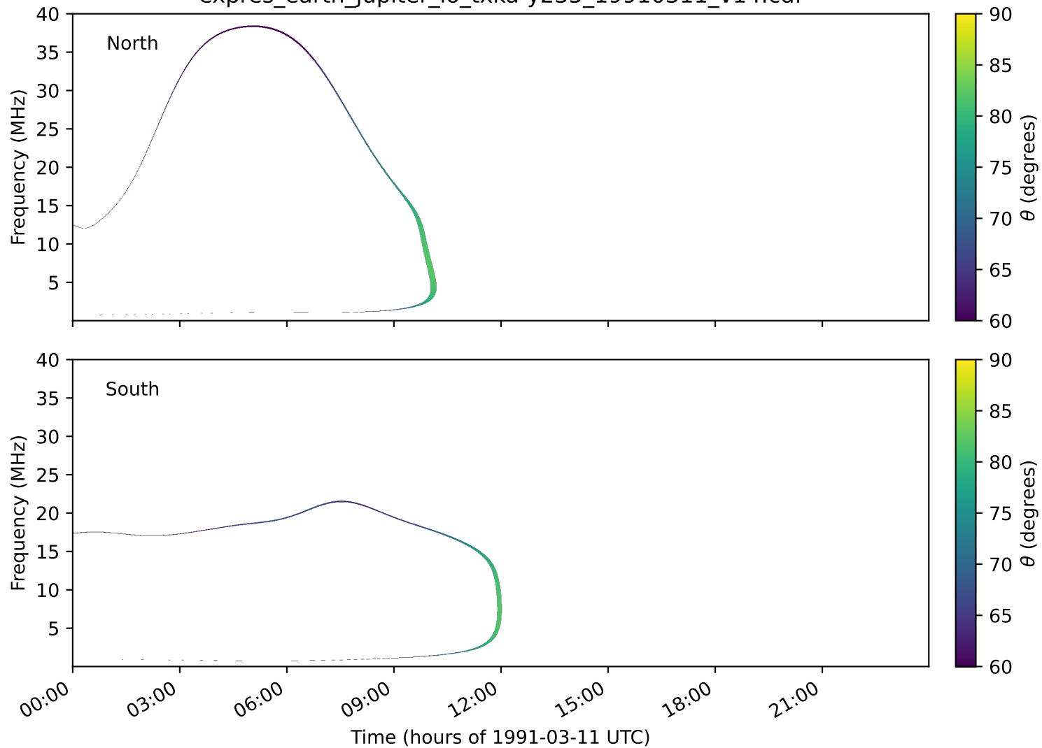
expres_earth_jupiter_io_txka-y235_19910311_v14.cdf
