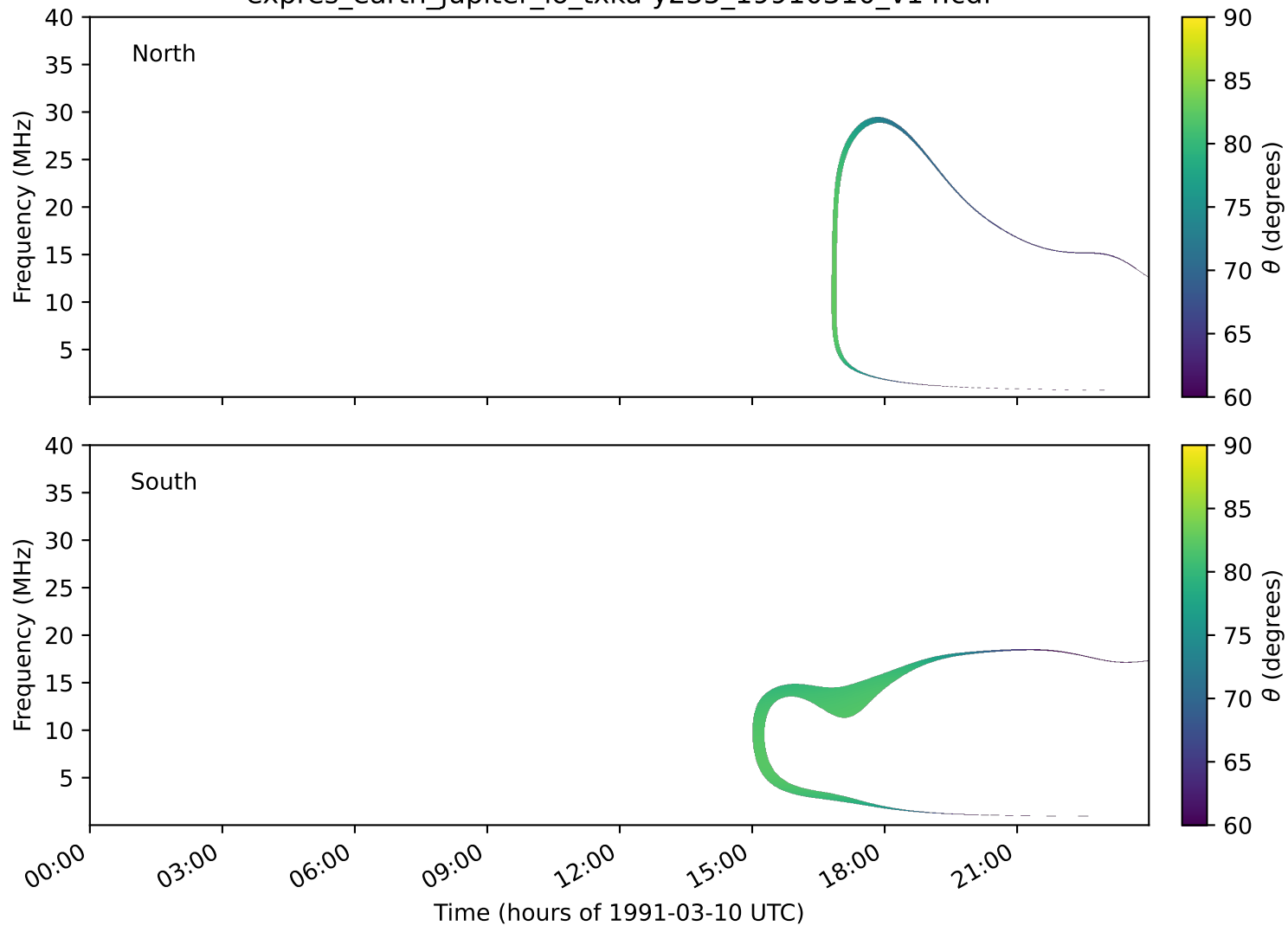
expres_earth_jupiter_io_txka-y235_19910310_v14.cdf
