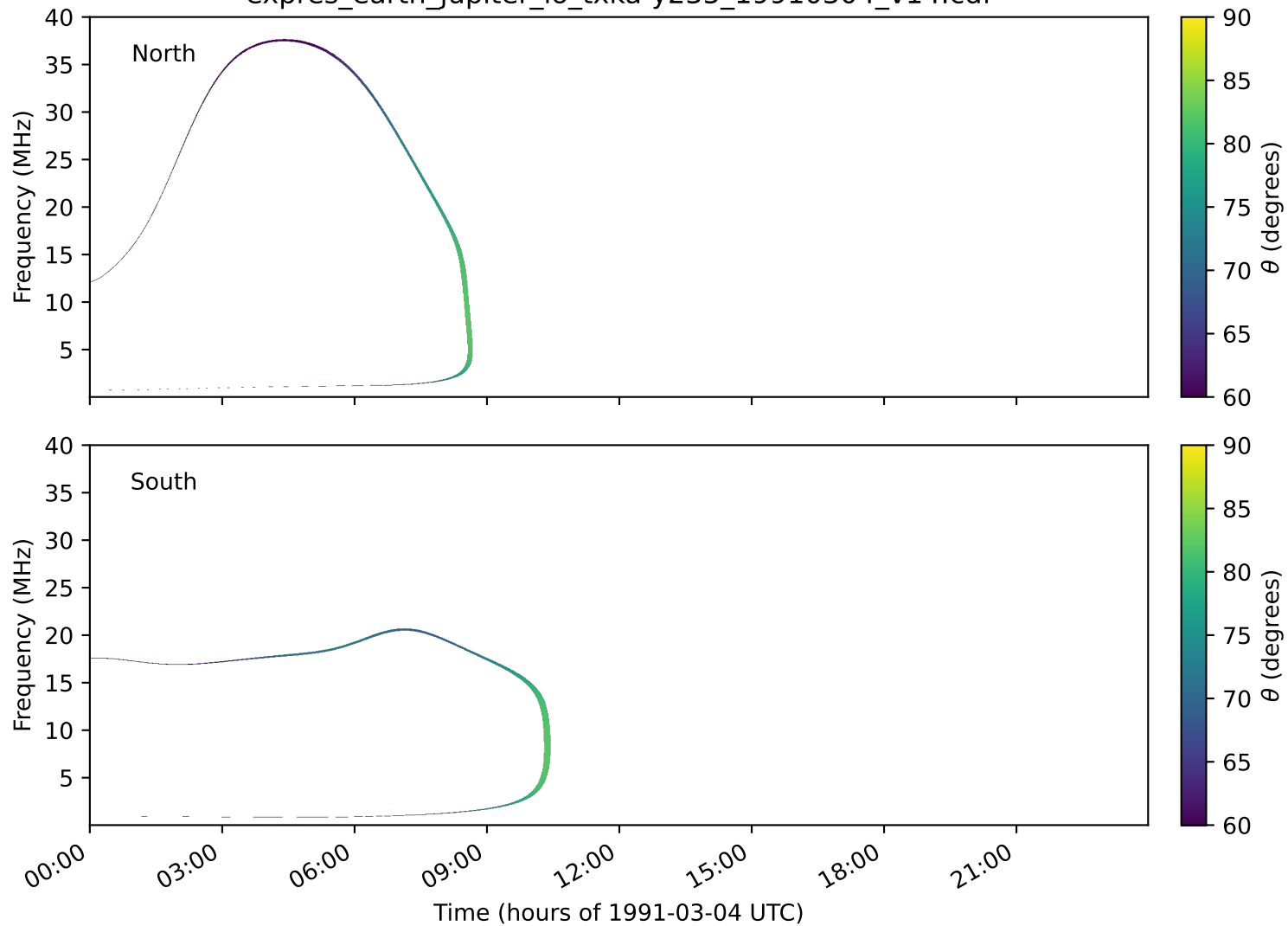
expres_earth_jupiter_io_txka-y235_19910304_v14.cdf
