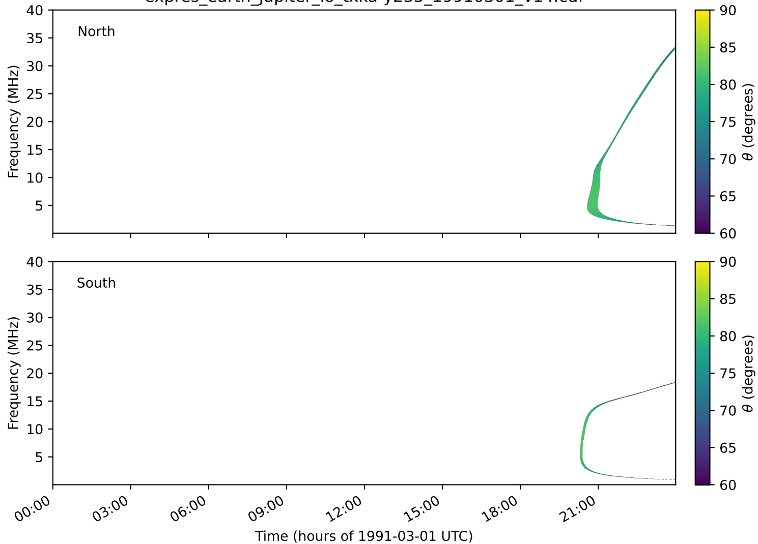
expres_earth_jupiter_io_txka-y235_19910301_v14.cdf
