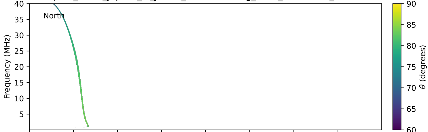
expres_earth_jupiter_io_jrm33_lossc-wid1deg_3kev_19910329_v11.cdf
