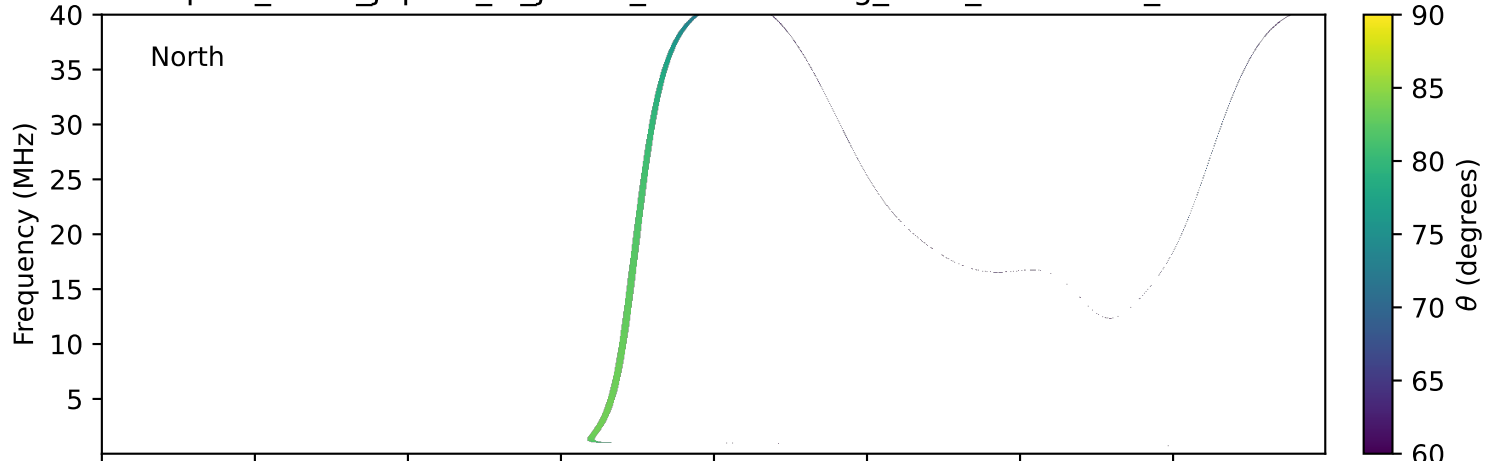
expres_earth_jupiter_io_jrm33_lossc-wid1deg_3kev_19910328_v11.cdf
