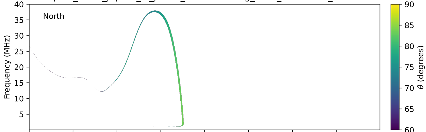
expres_earth_jupiter_io_jrm33_lossc-wid1deg_3kev_19910327_v11.cdf
