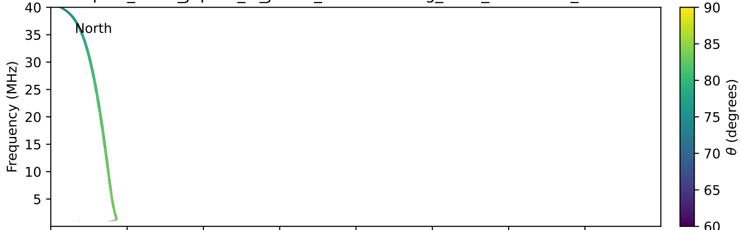
expres_earth_jupiter_io_jrm33_lossc-wid1deg_3kev_19910322_v11.cdf
