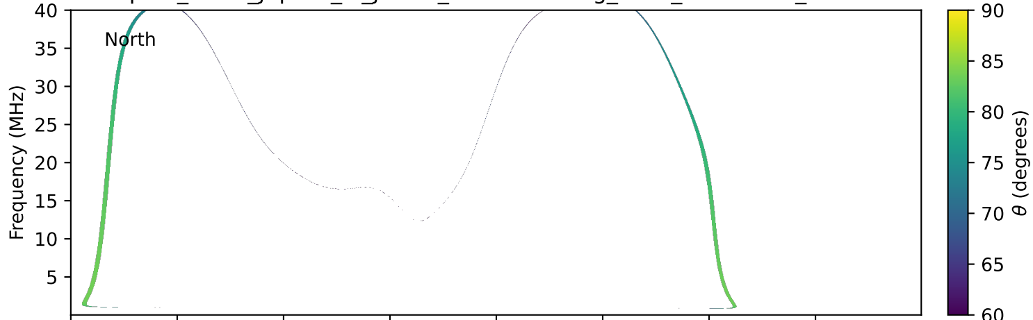
expres_earth_jupiter_io_jrm33_lossc-wid1deg_3kev_19910316_v11.cdf
