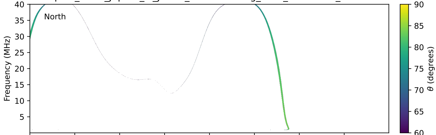
expres_earth_jupiter_io_jrm33_lossc-wid1deg_3kev_19910309_v11.cdf
