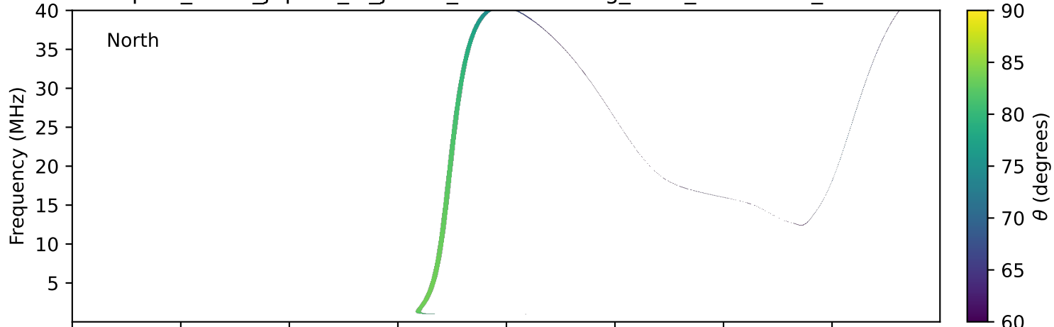
expres_earth_jupiter_io_jrm09_lossc-wid1deg_3kev_19910328_v11.cdf
