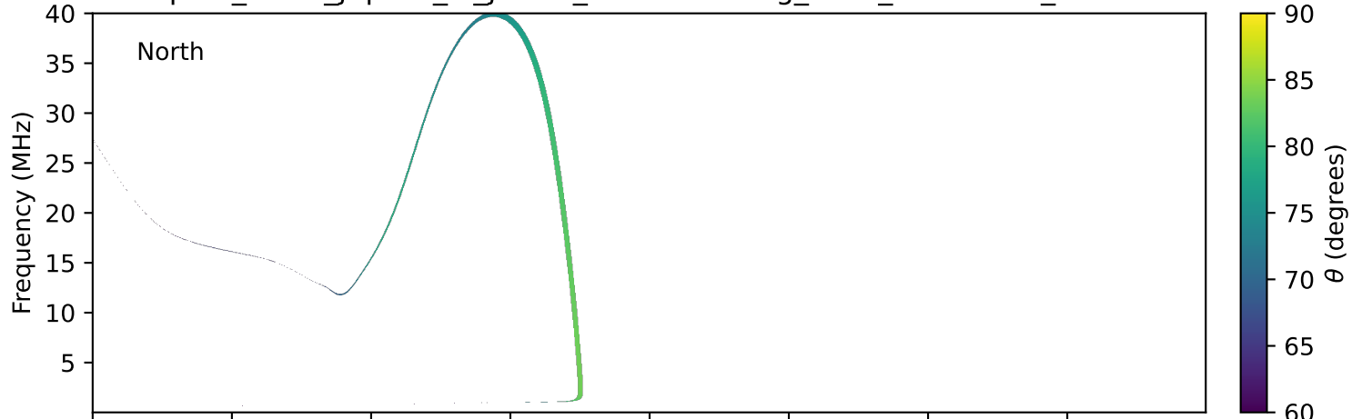
expres_earth_jupiter_io_jrm09_lossc-wid1deg_3kev_19910327_v11.cdf
