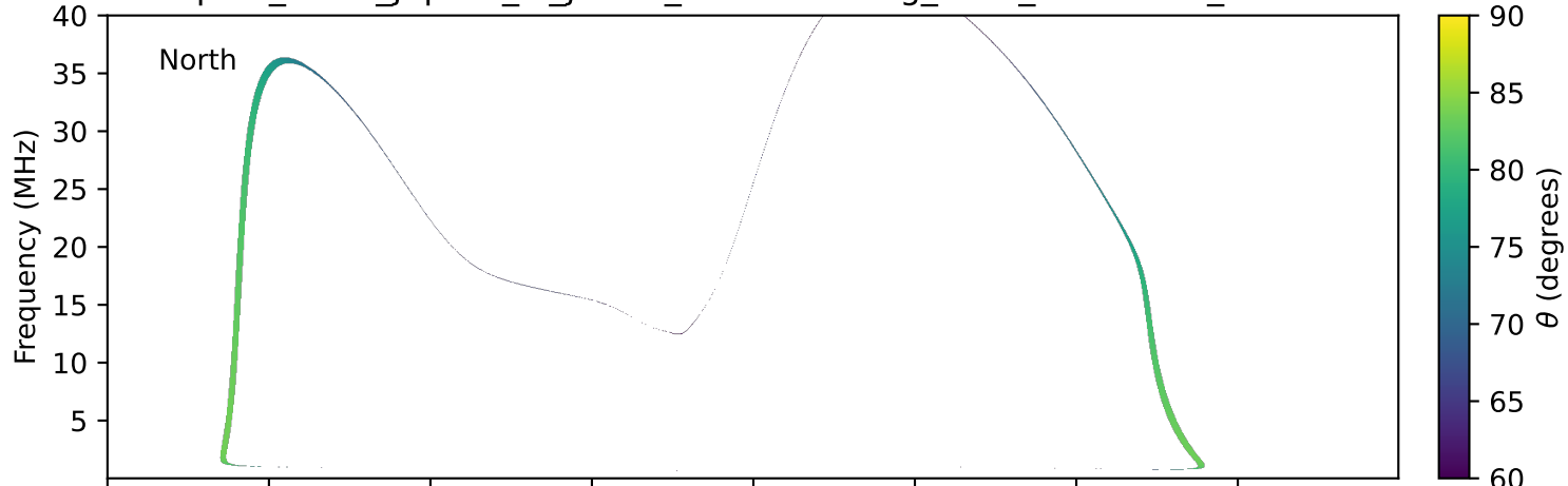
expres_earth_jupiter_io_jrm09_lossc-wid1deg_3kev_19910323_v11.cdf
