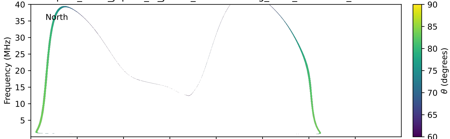
expres_earth_jupiter_io_jrm09_lossc-wid1deg_3kev_19910316_v11.cdf
