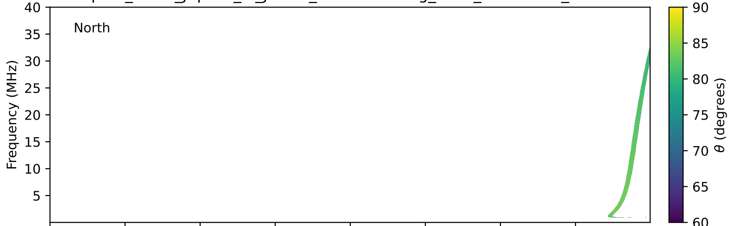
expres_earth_jupiter_io_jrm09_lossc-wid1deg_3kev_19910308_v11.cdf
