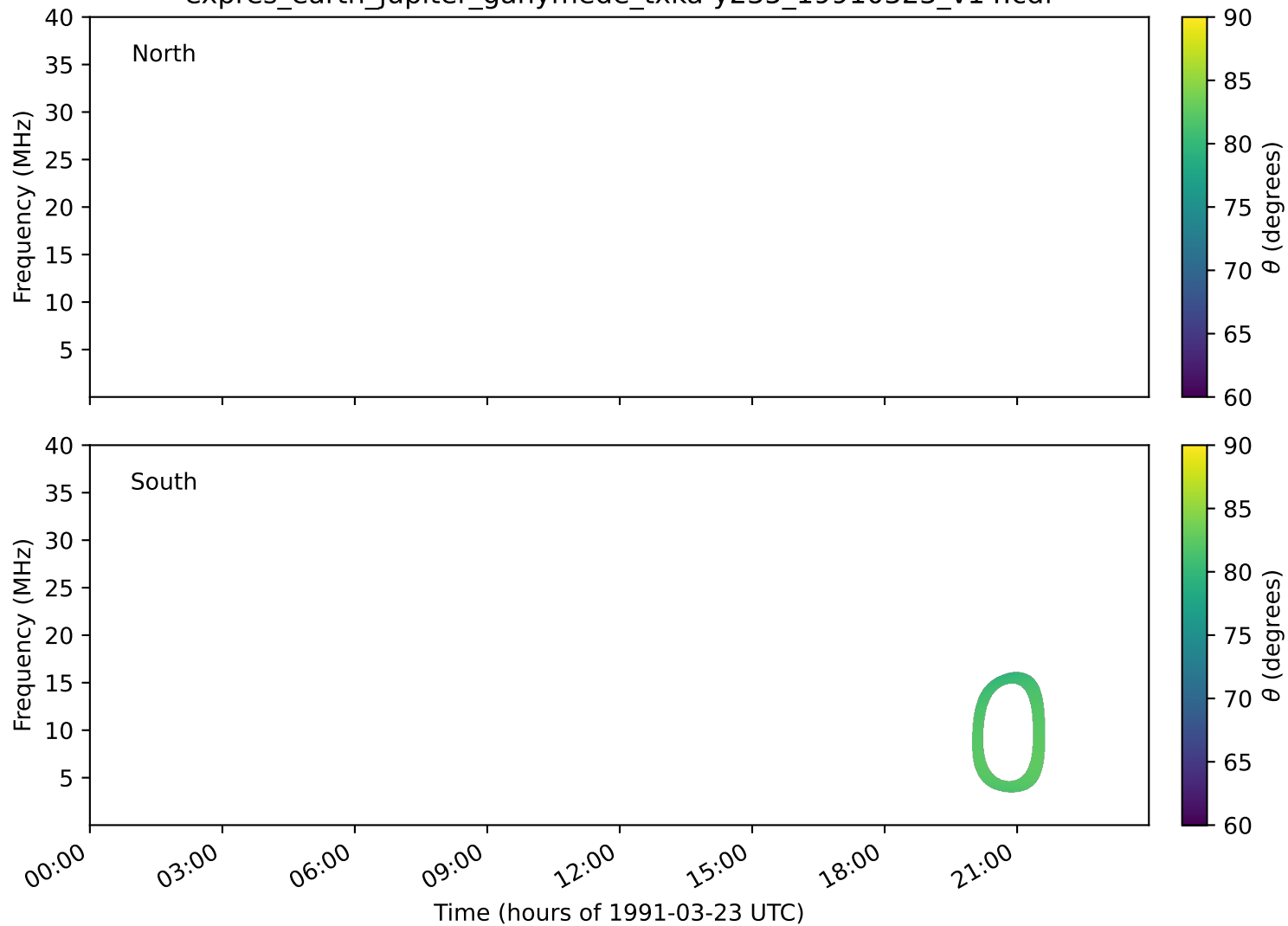
expres_earth_jupiter_ganymede_txka-y235_19910323_v14.cdf
