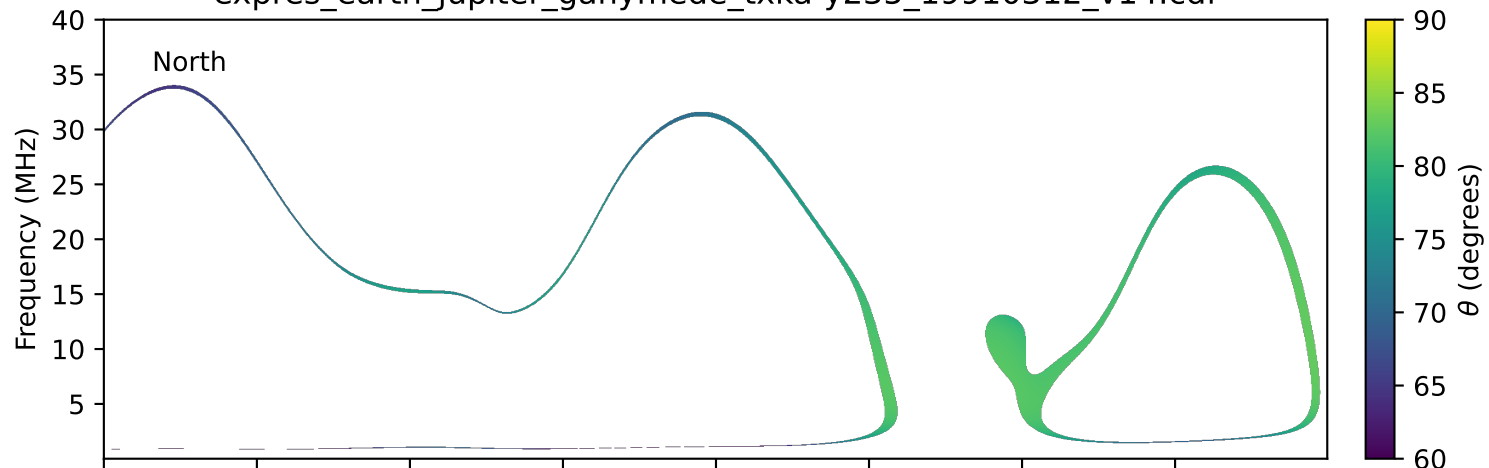
expres_earth_jupiter_ganymede_txka-y235_19910312_v14.cdf
