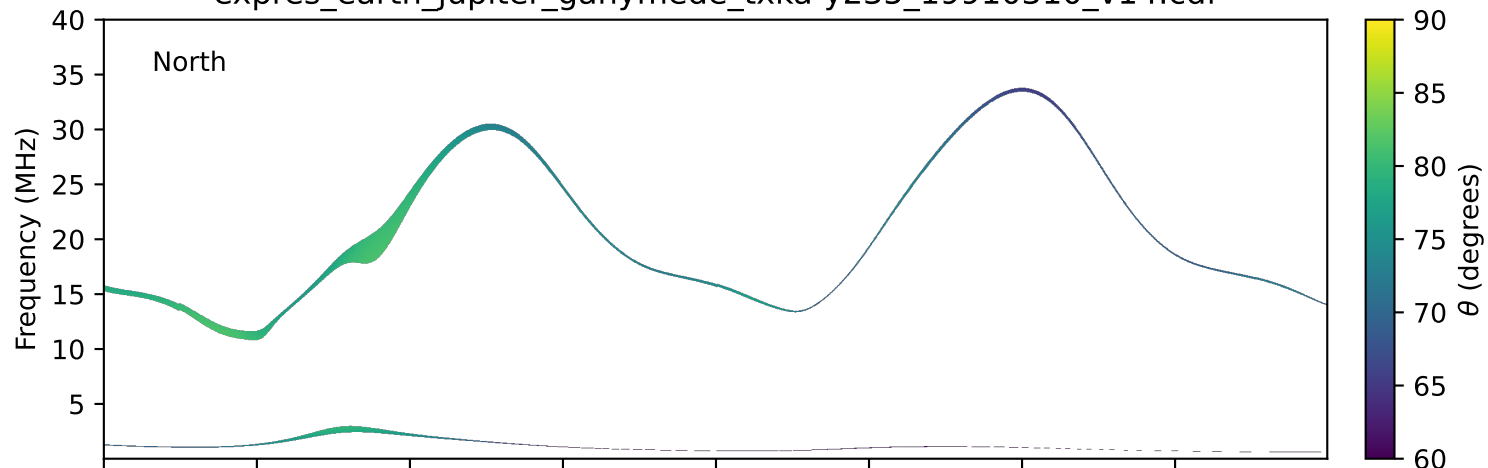
expres_earth_jupiter_ganymede_txka-y235_19910310_v14.cdf
