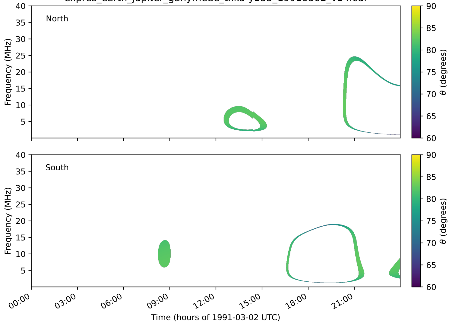
expres_earth_jupiter_ganymede_txka-y235_19910302_v14.cdf
