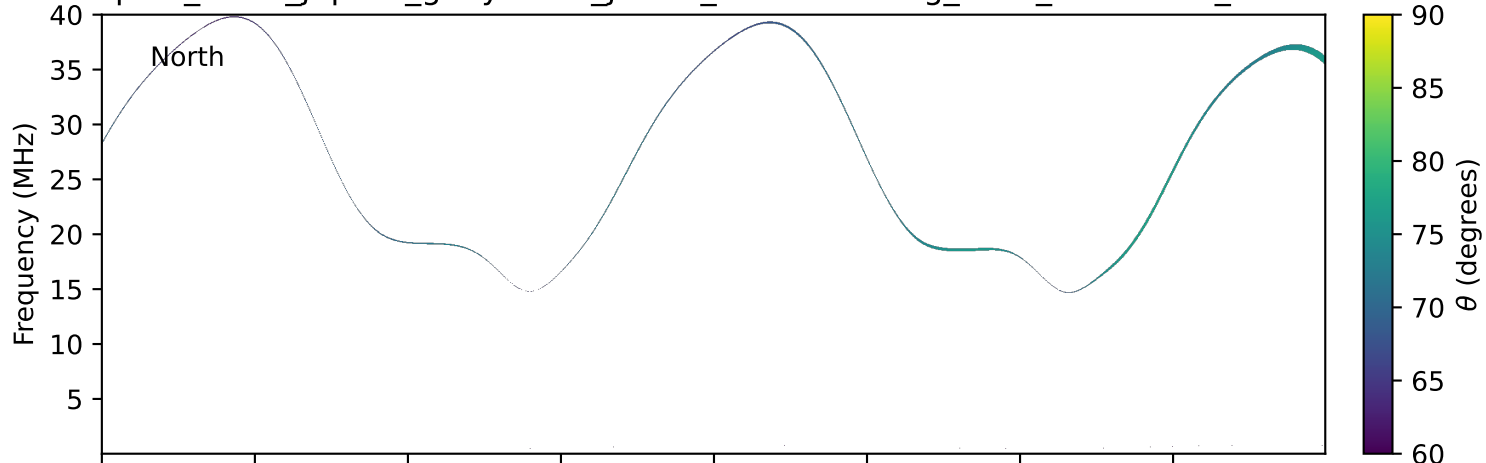
expres_earth_jupiter_ganymede_jrm33_lossc-wid1deg_3kev_19910326_v11.cdf
