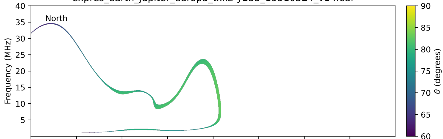
expres_earth_jupiter_europa_txka-y235_19910324_v14.cdf
