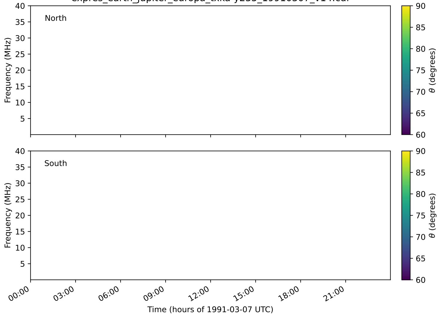
expres_earth_jupiter_europa_txka-y235_19910307_v14.cdf
