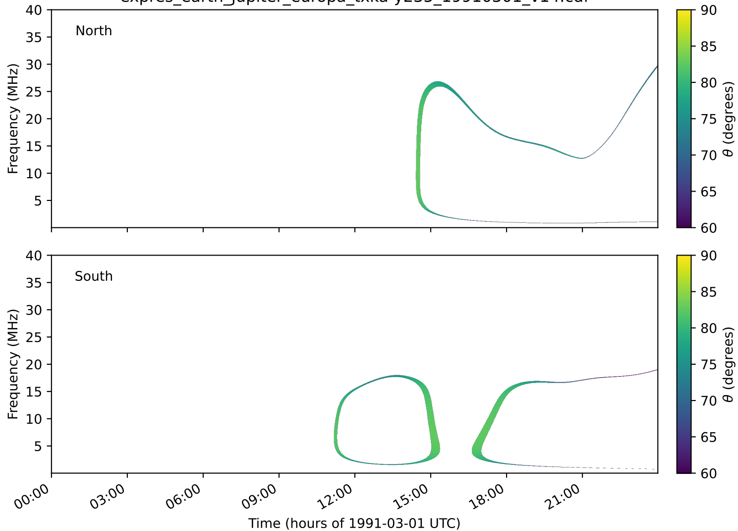
expres_earth_jupiter_europa_txka-y235_19910301_v14.cdf
