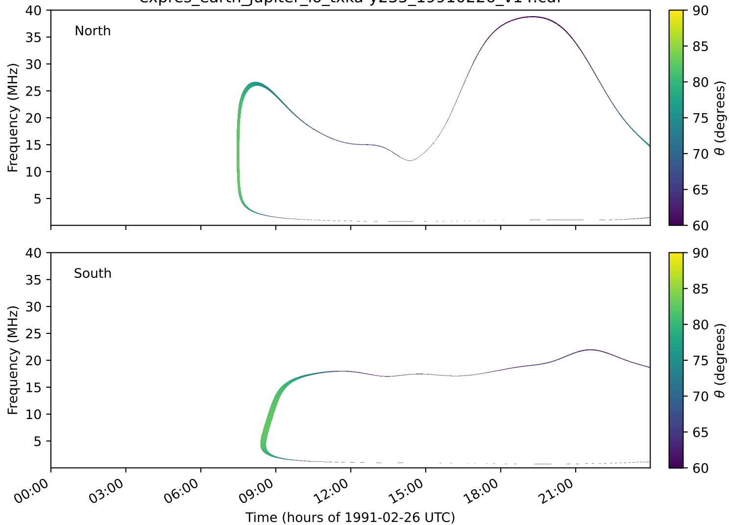
expres_earth_jupiter_io_txka-y235_19910226_v14.cdf
