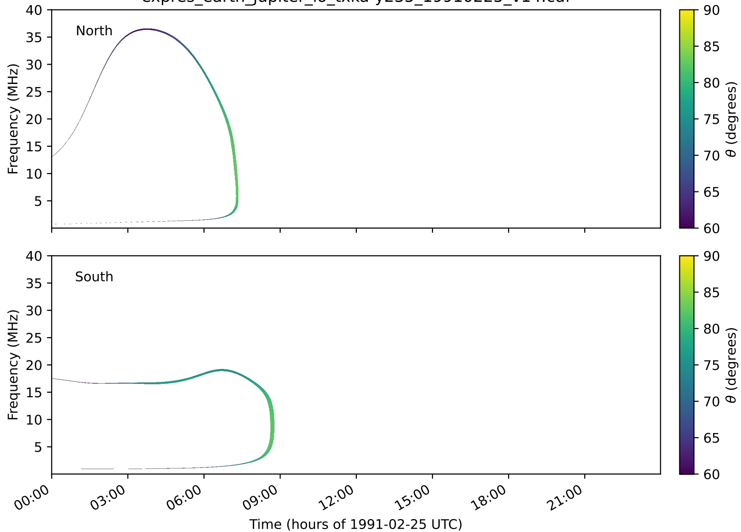
expres_earth_jupiter_io_txka-y235_19910225_v14.cdf
