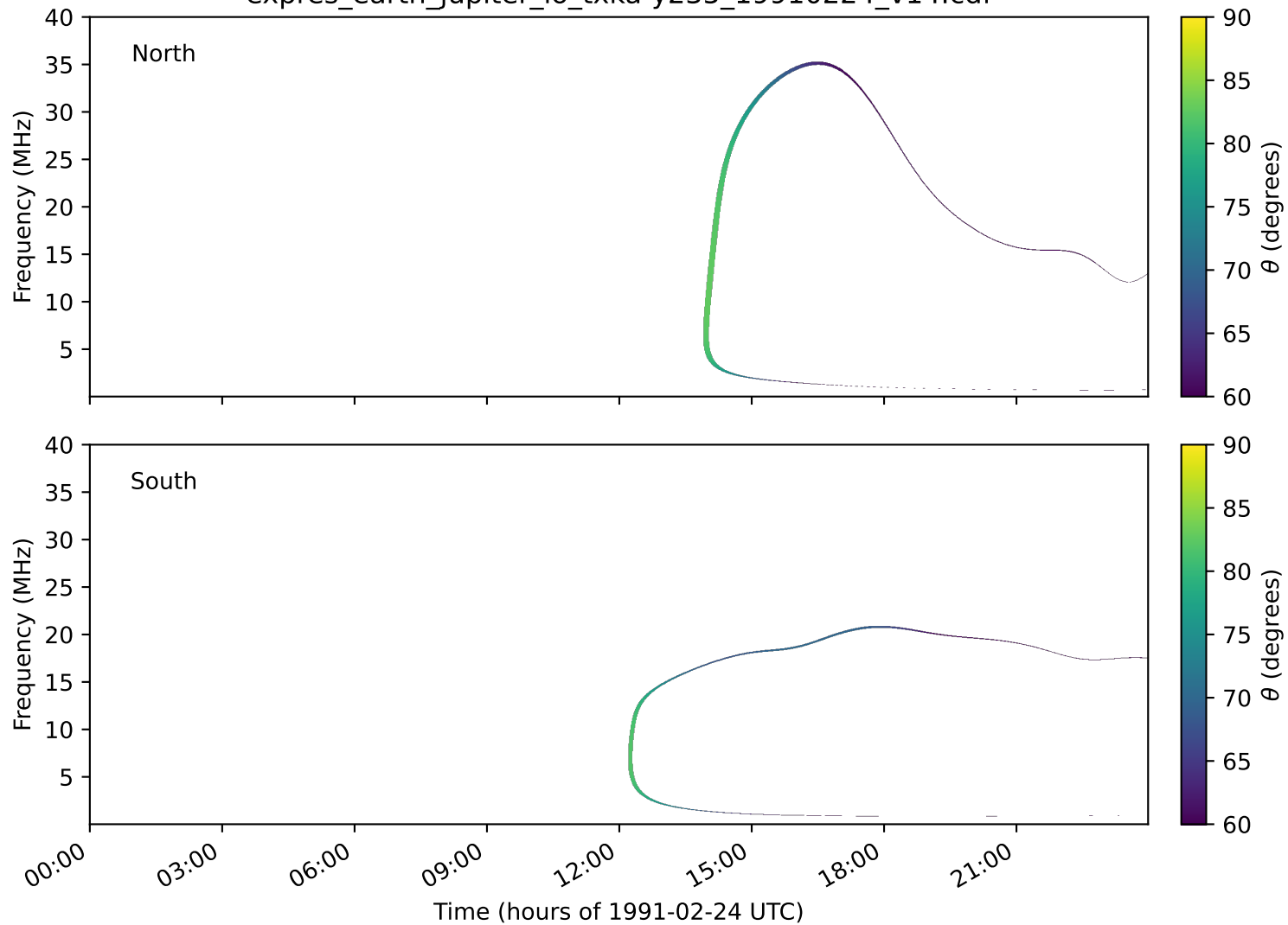
expres_earth_jupiter_io_txka-y235_19910224_v14.cdf
